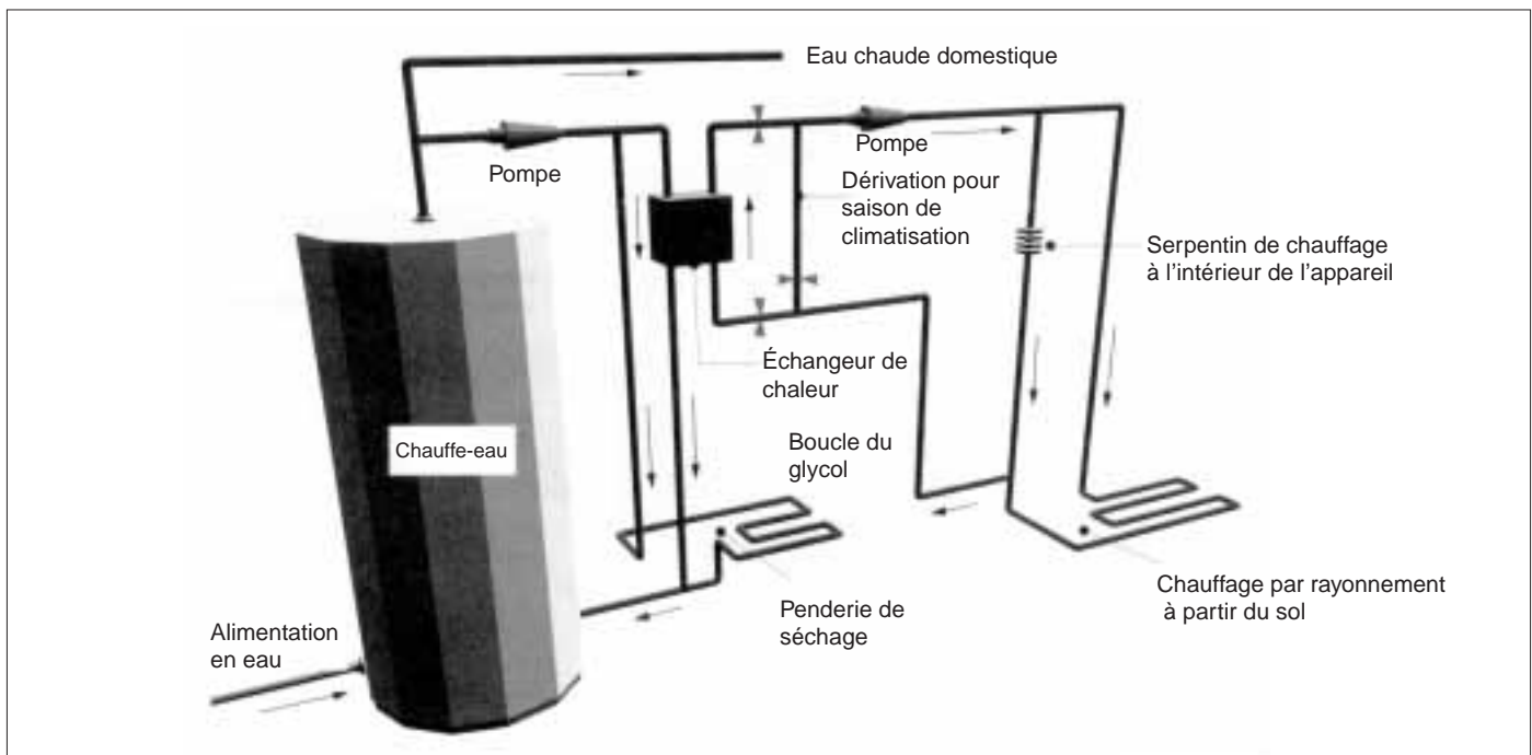
Figure 10 : Installation de chauffage
