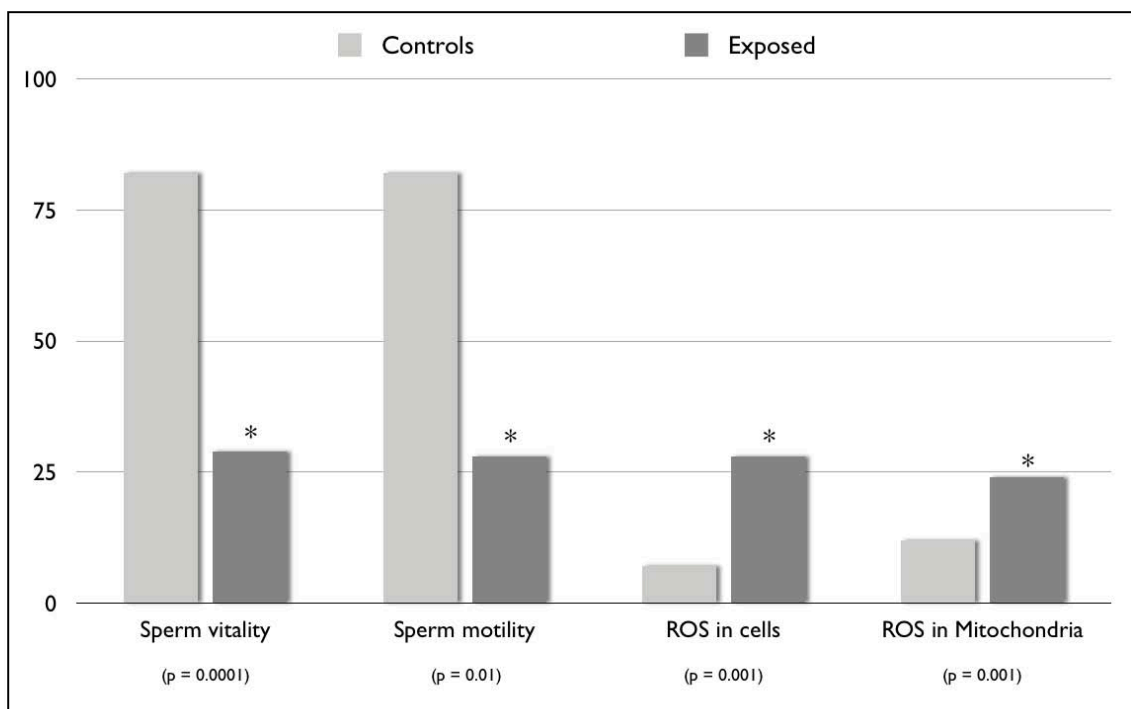
Figure 11: Sperm exposed in vitro to 1.8 GHz (SAR = 27.5 W/kg) for 16 hours @ 21°C (isothermal conditions). (De Iuliis et al., 2009)
