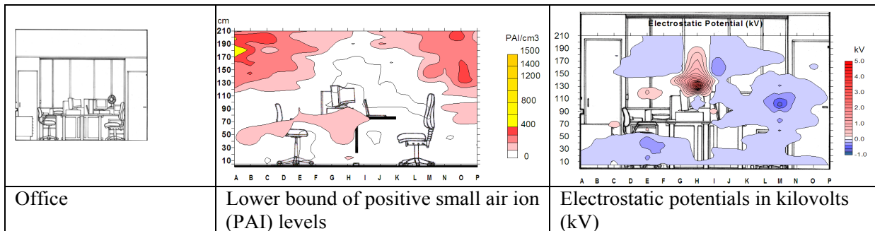
Figure 2b. Vertical Section through Office Environment. Adapted from [19].
