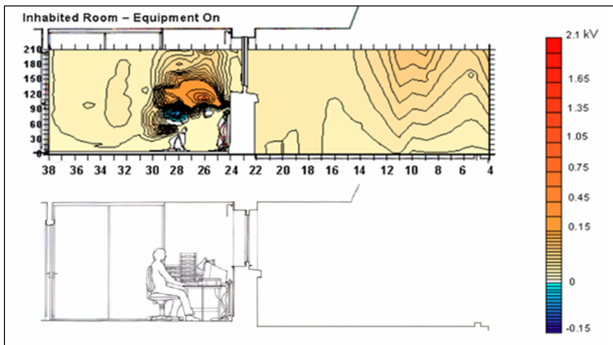
Figure 1. Electrostatic potentials measured indoors and outdoors. (Jamieson – unpublished research).
